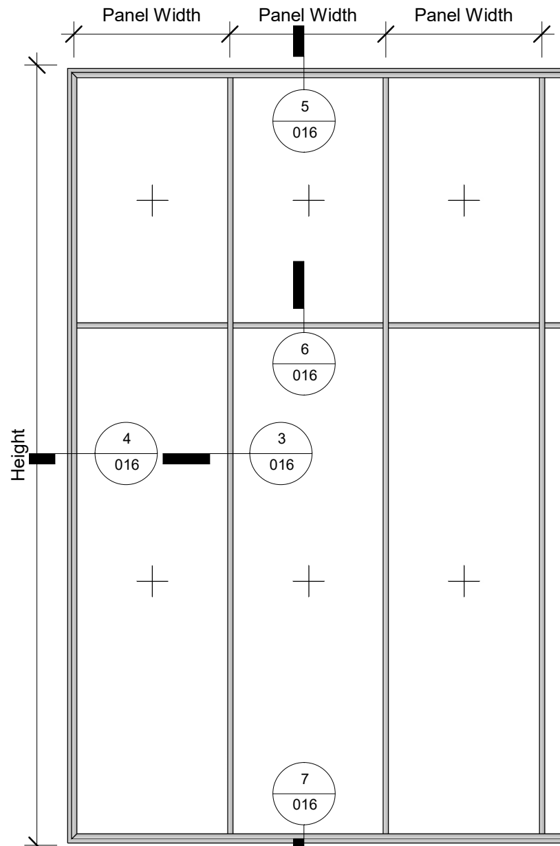
1 Elevation Front 1 : 20
